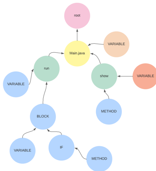
Fig. 1. Sample source code and its AST.
