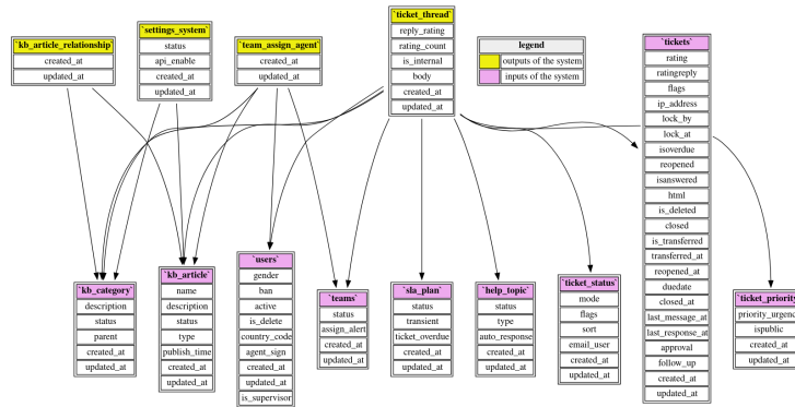
Fig. 4. Metamodel of the Faveo information system
