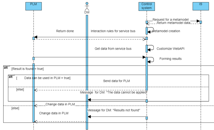
Fig. 7. The process of organizing interaction and maintaining the system in a state of operability with the participation of the management system and the decision maker
